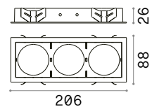
SQUARE - FRAME TRIPLE Required
