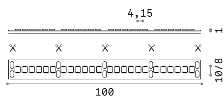
SMD 2835 240 LED/m - 50.000 h
