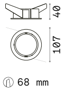
ROUND - FRAME SINGLE Required
