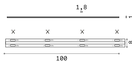
COB 180 LED/m - 50.000h
